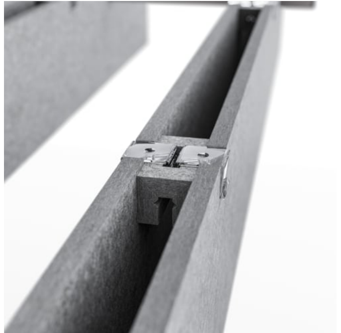
Box Baffle Span - Clip Brace Detail
